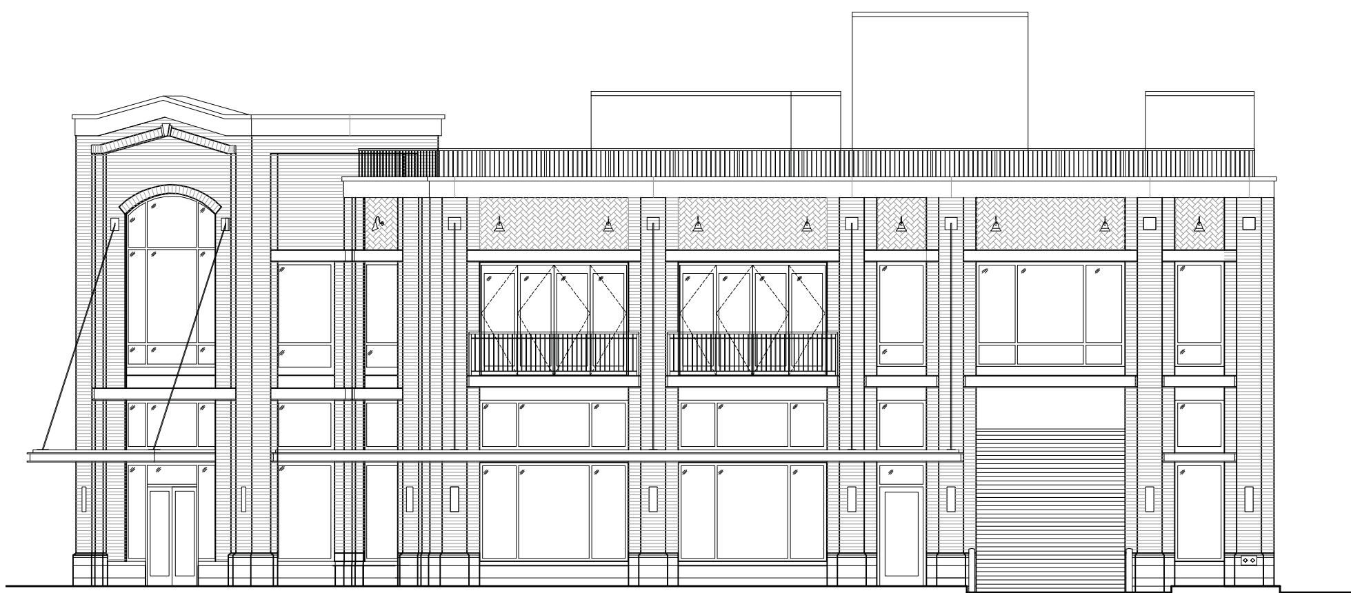
15th Street Elevation
