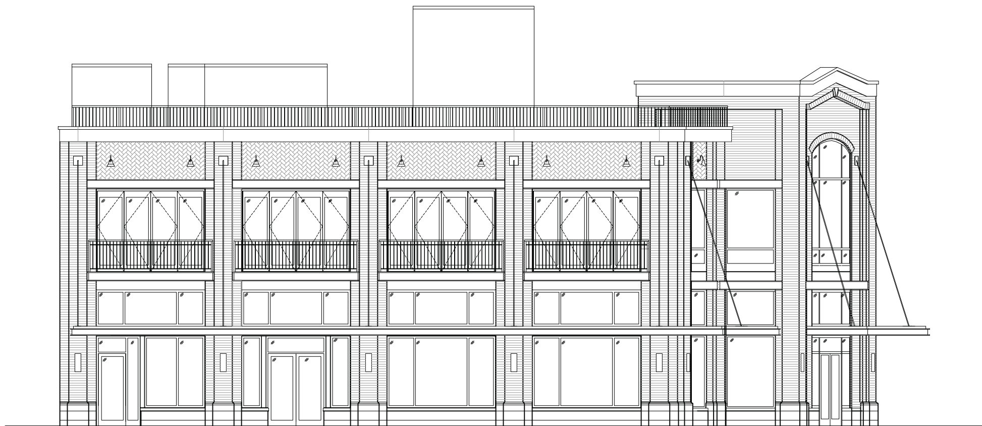
Pennsylvania Avenue Elevation
