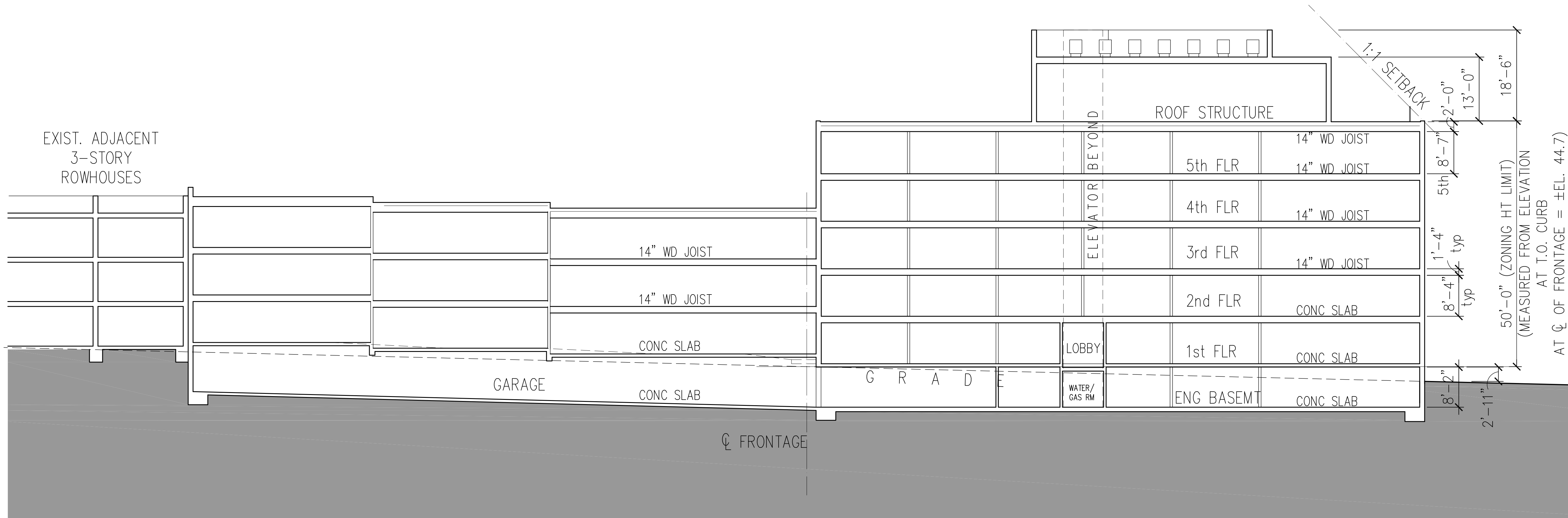
EAST - WEST SECTION (LOOKING NORTH)
